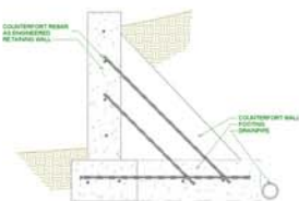
CONCRETE COUNTERFORT
