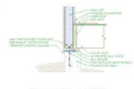
SIP PANEL AT SILL
