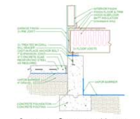
GARAGE SLAB AT HOUSE
