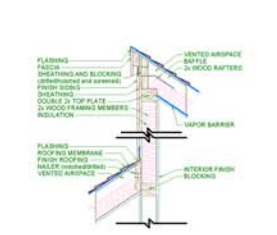
SHED ROOF PEAK AND WALL INTERSECTION
