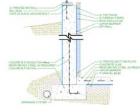
BASEMENT FOUNDATION
