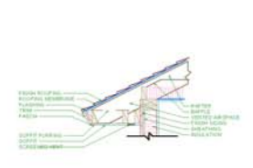
VENTED SOFFIT
