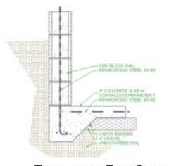
THICKENED END SLAB BELOW GRADE
