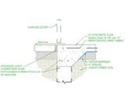
TURNED DOWN SLAB AT GARAGE
