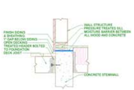
DECK ANCHORED TO FOUNDATION
