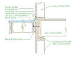
WATERPROOF DECK
