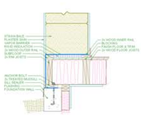
STRAW BALE ON FOUNDATION
