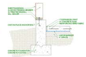
CONCRETE SLAB AT GARAGE FOUNDATION
