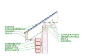
EAVE AT BRICK VENEER
