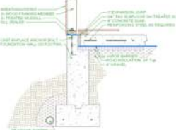
CONCRETE SLAB ON GRADE
