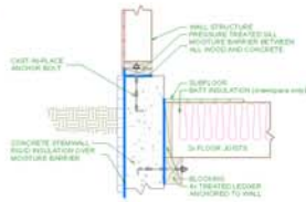
JOISTS BELOW MUDSILL
