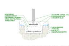
ADJUSTABLE COLUMN ON PIER
