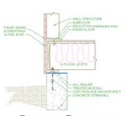
FLOOR AT FOUNDATION
