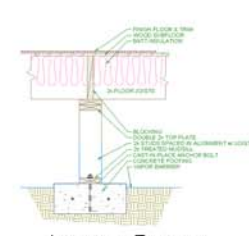
INTERIOR FOOTING
